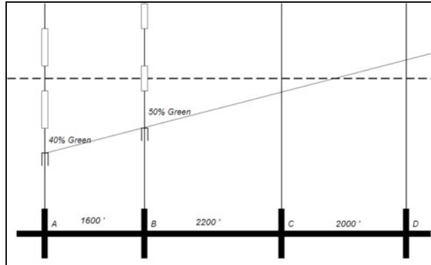
Figure . Kell Method (continued)
