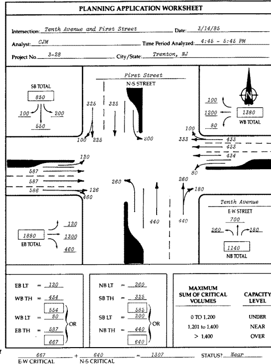
Figure 6. Critical Lane Analysis Example.
