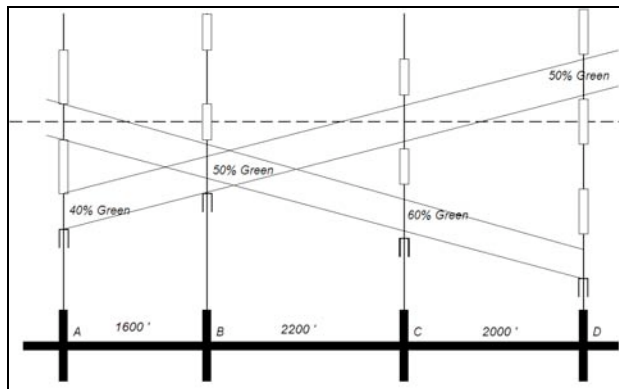
Figure 5 . Kell Method (Completed Diagram).
